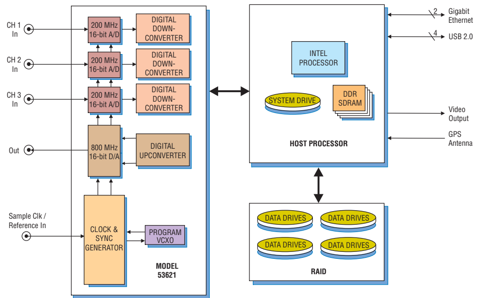
MODEL RTX 2786 Three Record Channels and One Playback Channel. Contact Pentek for Other Configurations.
